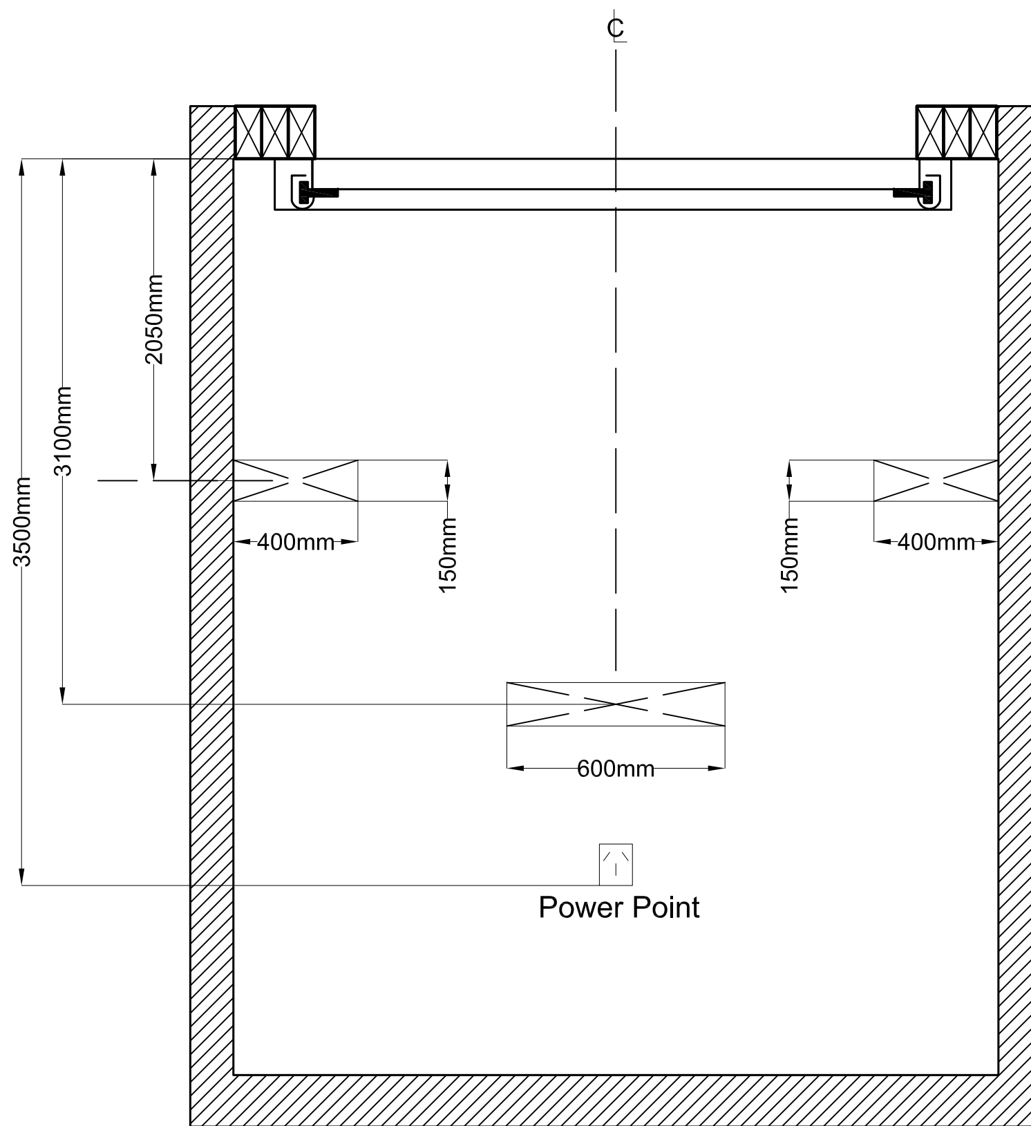
NOGGING DETAIL FOR SECTIONAL UP TO 2.3M HIGH (TRACK AND MOTOR FIXINGS)
