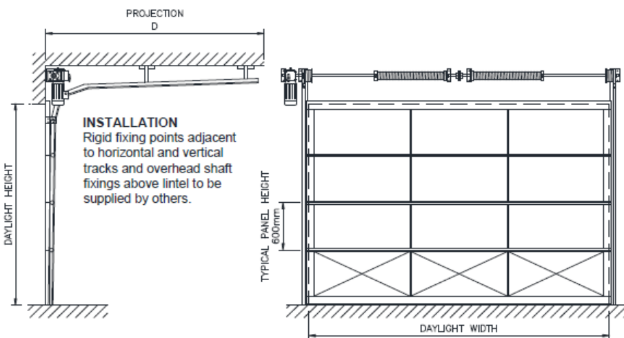
SIDE ELEVATION
